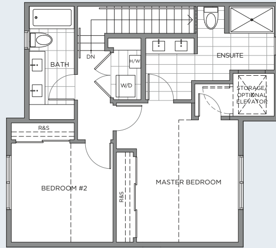
LEVEL 3 PLAN - 743 SQ FT
