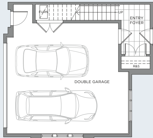
LEVEL 1 PLAN - 141 SQ FT
