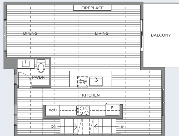
LEVEL 2 PLAN - 694 SQ FT
