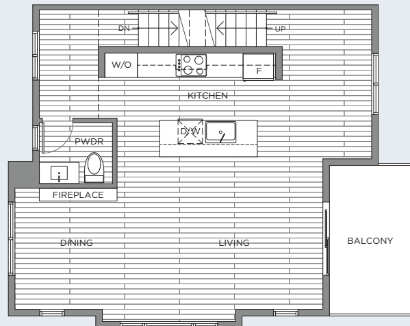
LEVEL 2 PLAN - 711 SQ FT
