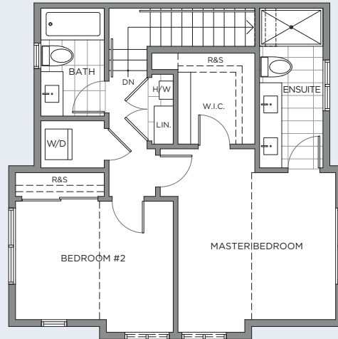
LEVEL 3 PLAN - 645 SQ FT
