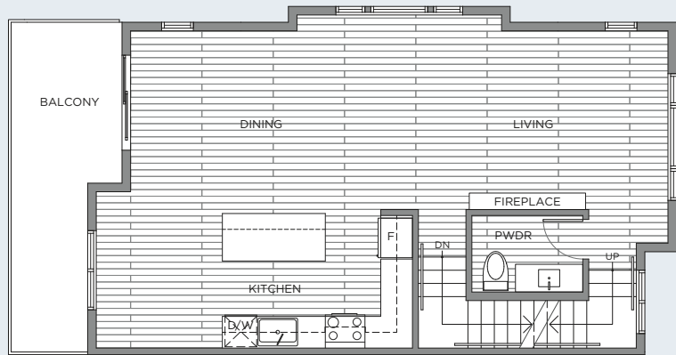
LEVEL 2 PLAN - 760 SQ FT
