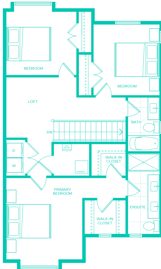
LEVEL 2 - 932 SQ FT
