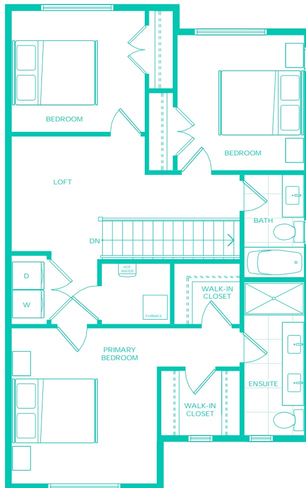
LEVEL 2 - 945 SQ FT
