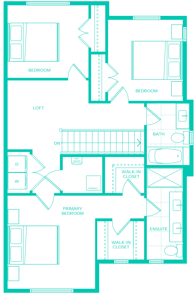
LEVEL 2 - 942 SQ FT
